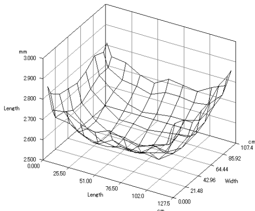
(Kraft) pressured thickness after one cycle
