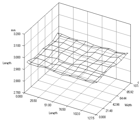
(YOM) pressured thickness after 200cycles
